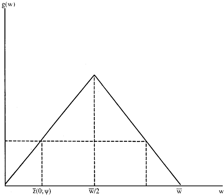
FIG. 4. Triangular distribution.
